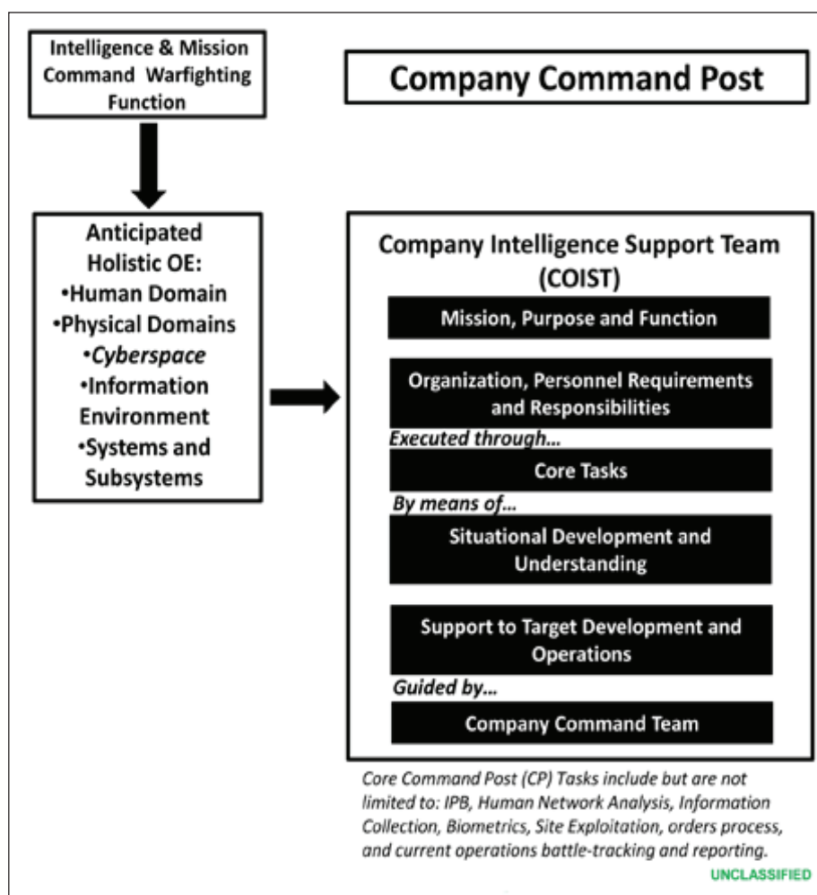
Figure 3. COIST Framework. 5
